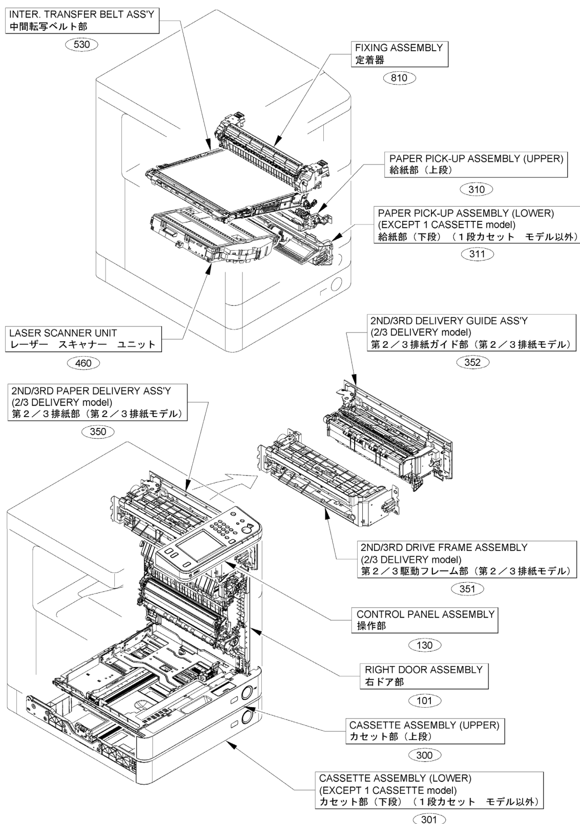
Figure A1 (1/3) ASSEMBLY LOCATION DIAGRAM
