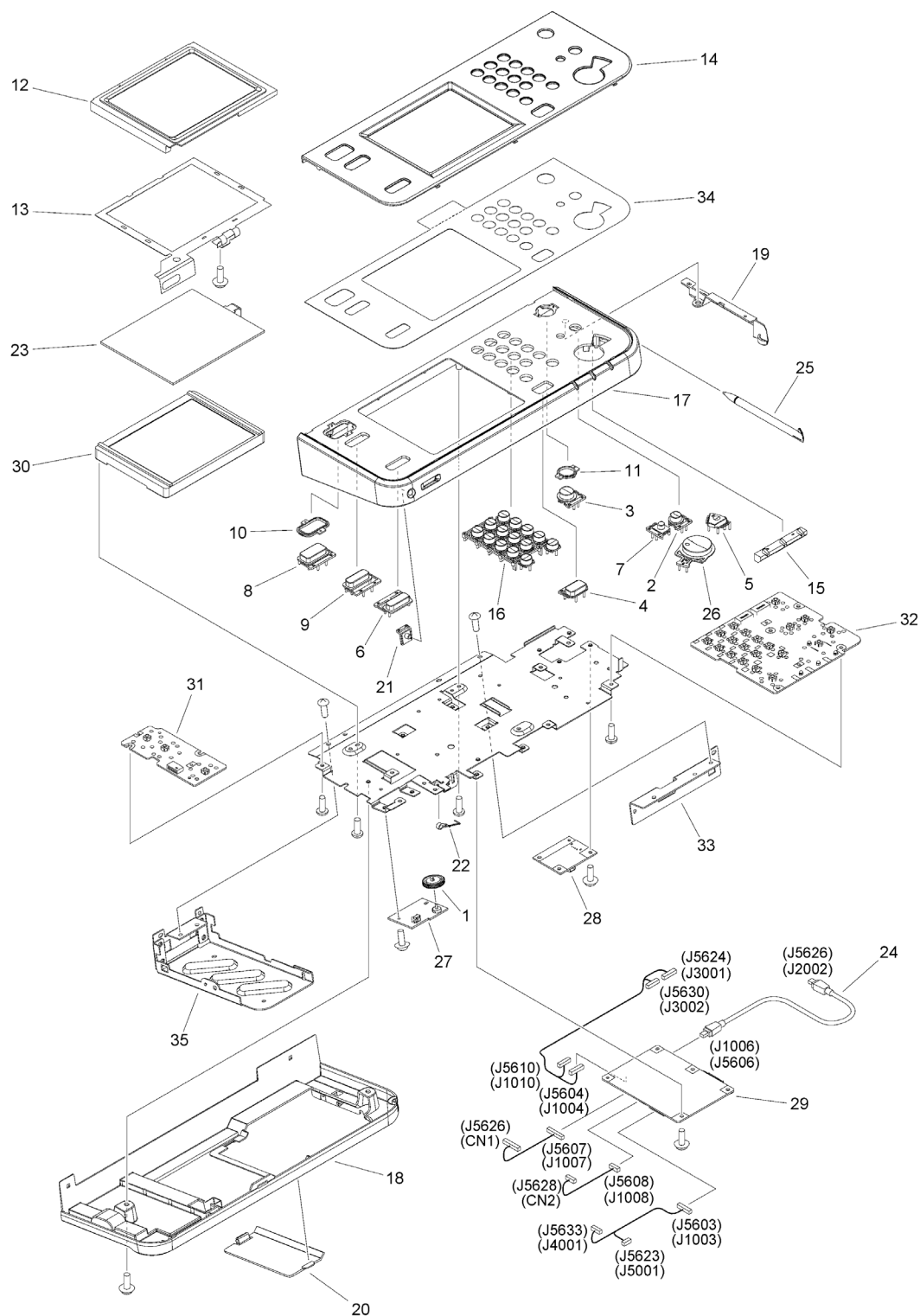
Figure 130 CONTROL PANEL ASSEMBLY
