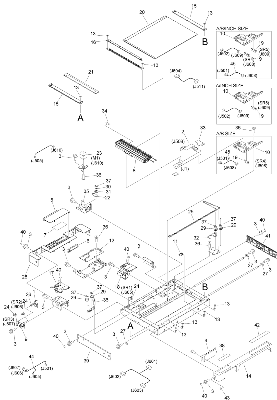
Figure D11 READER ASSEMBLY (EXCEPT EUR)
