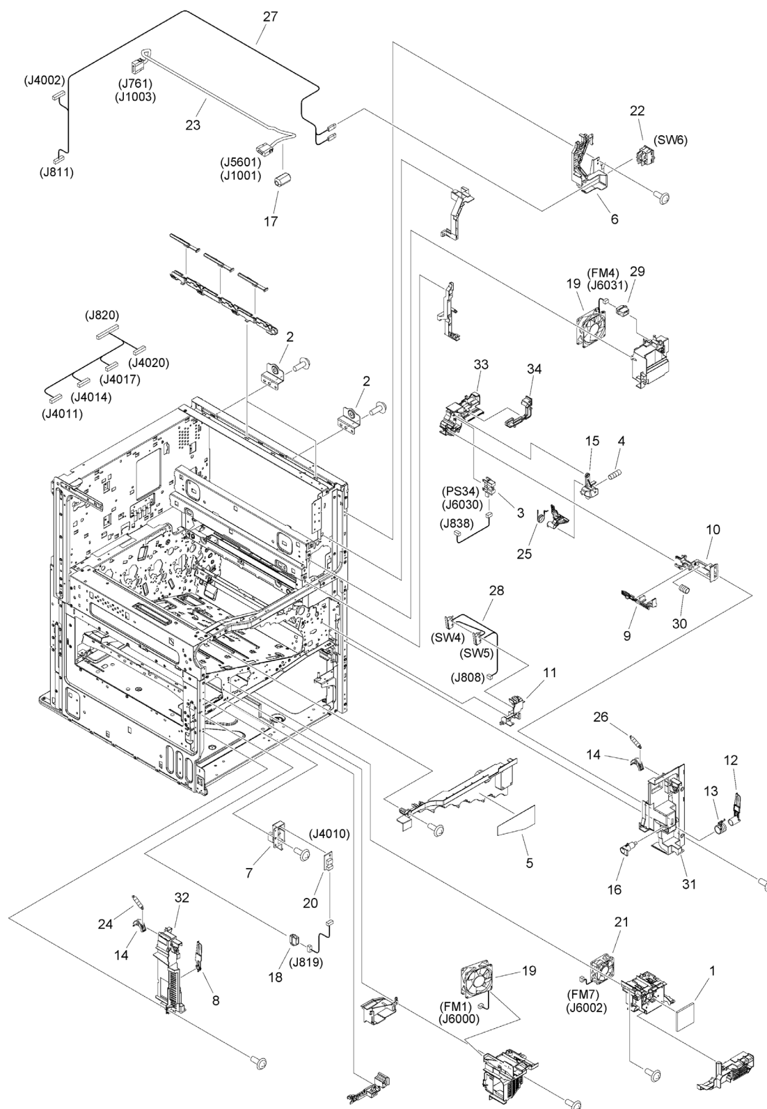
Figure 102 INTERNAL COMPONENTS 1
