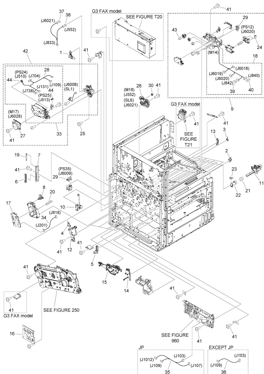
Figure 109 MACHINE REAR PLATE 2
