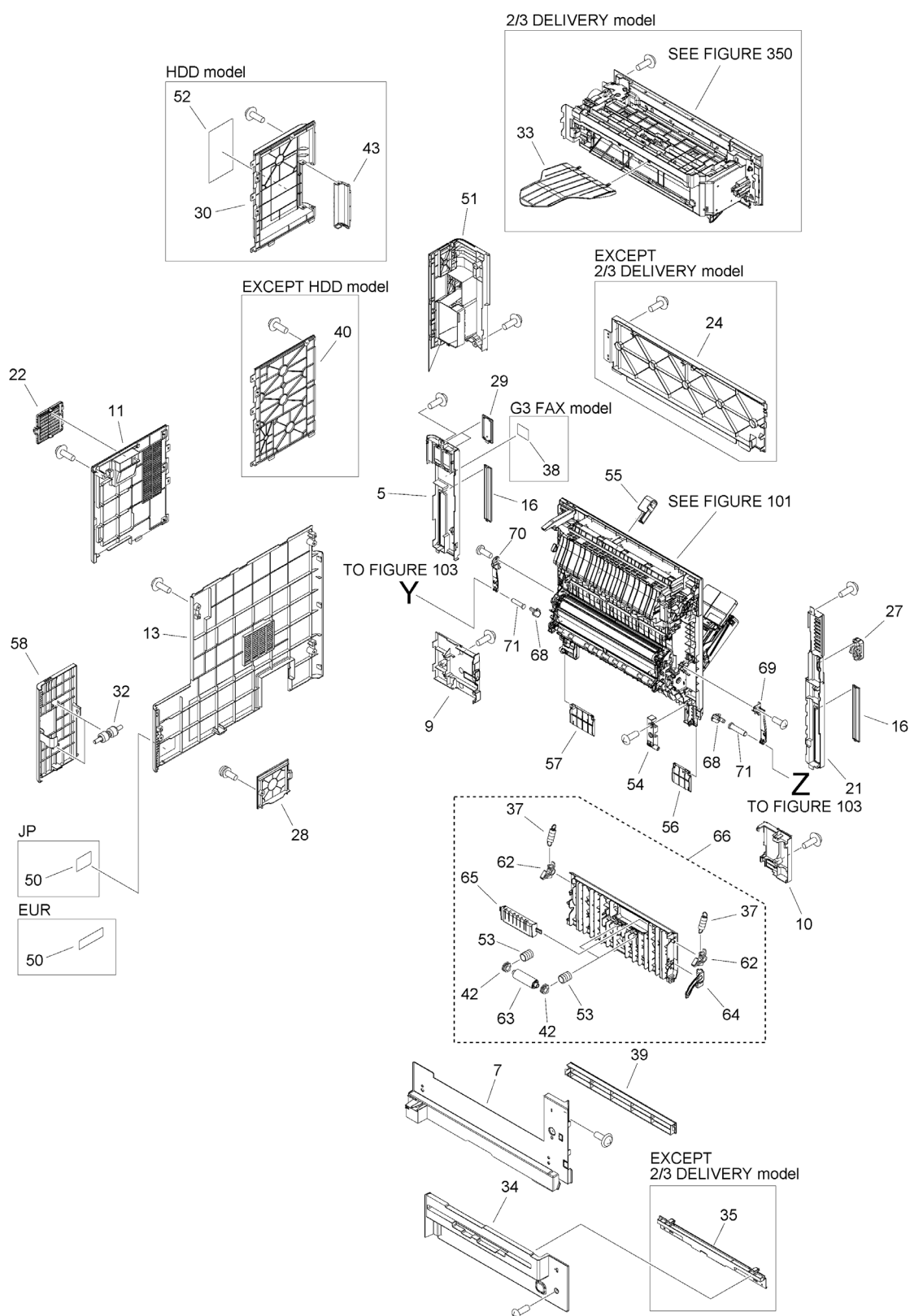
Figure 100 (2/2) EXTERNAL COVERS, PANELS, ETC.
