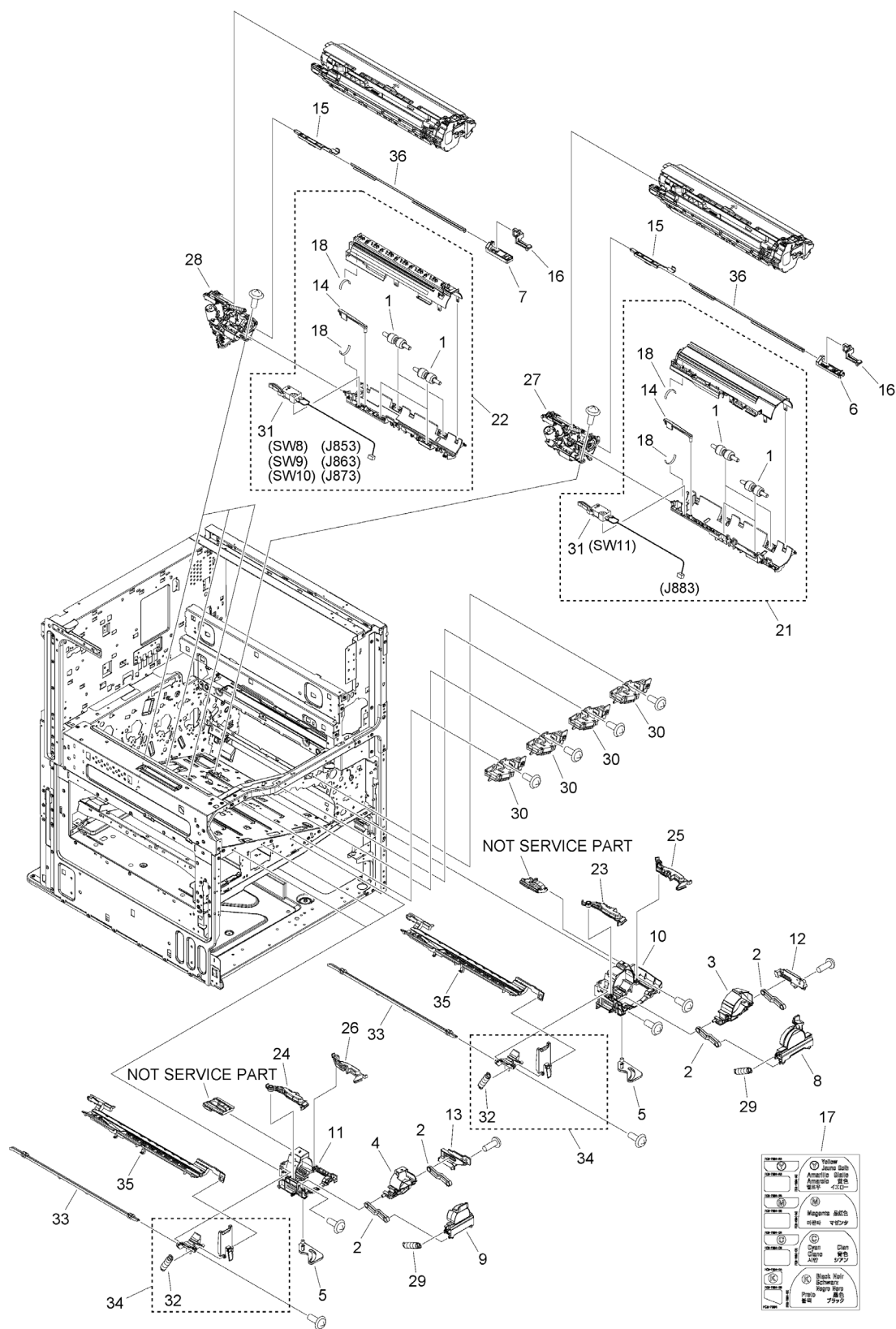
Figure 106 INTERNAL COMPONENTS 5
