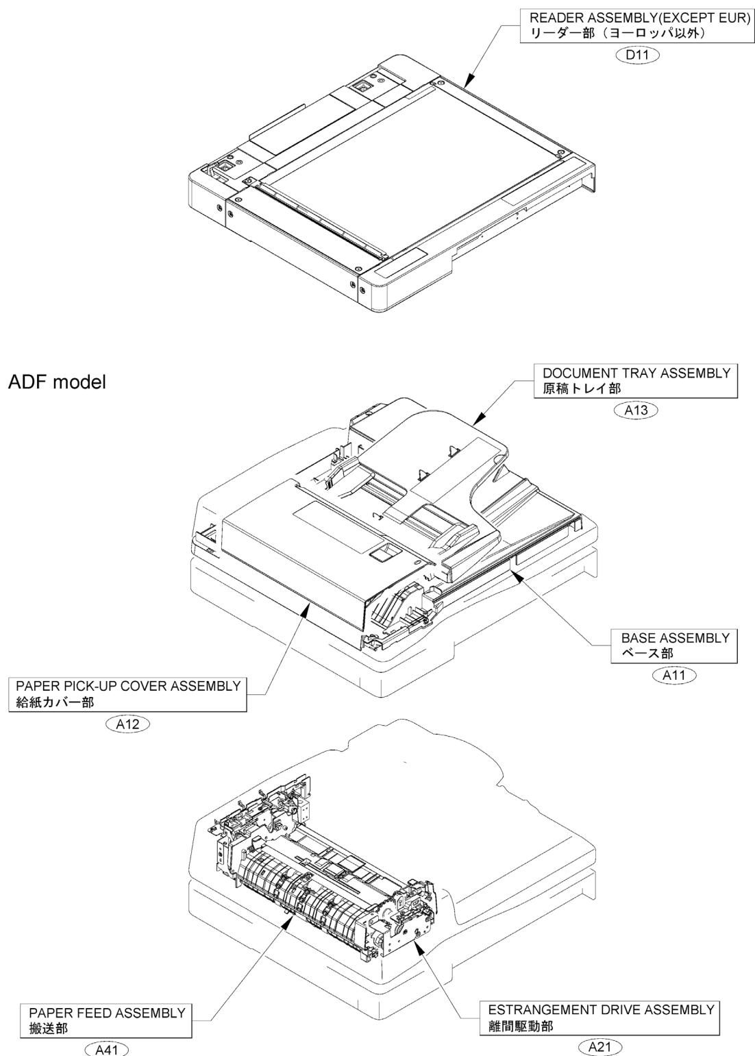
Figure A1 (3/3) ASSEMBLY LOCATION DIAGRAM
