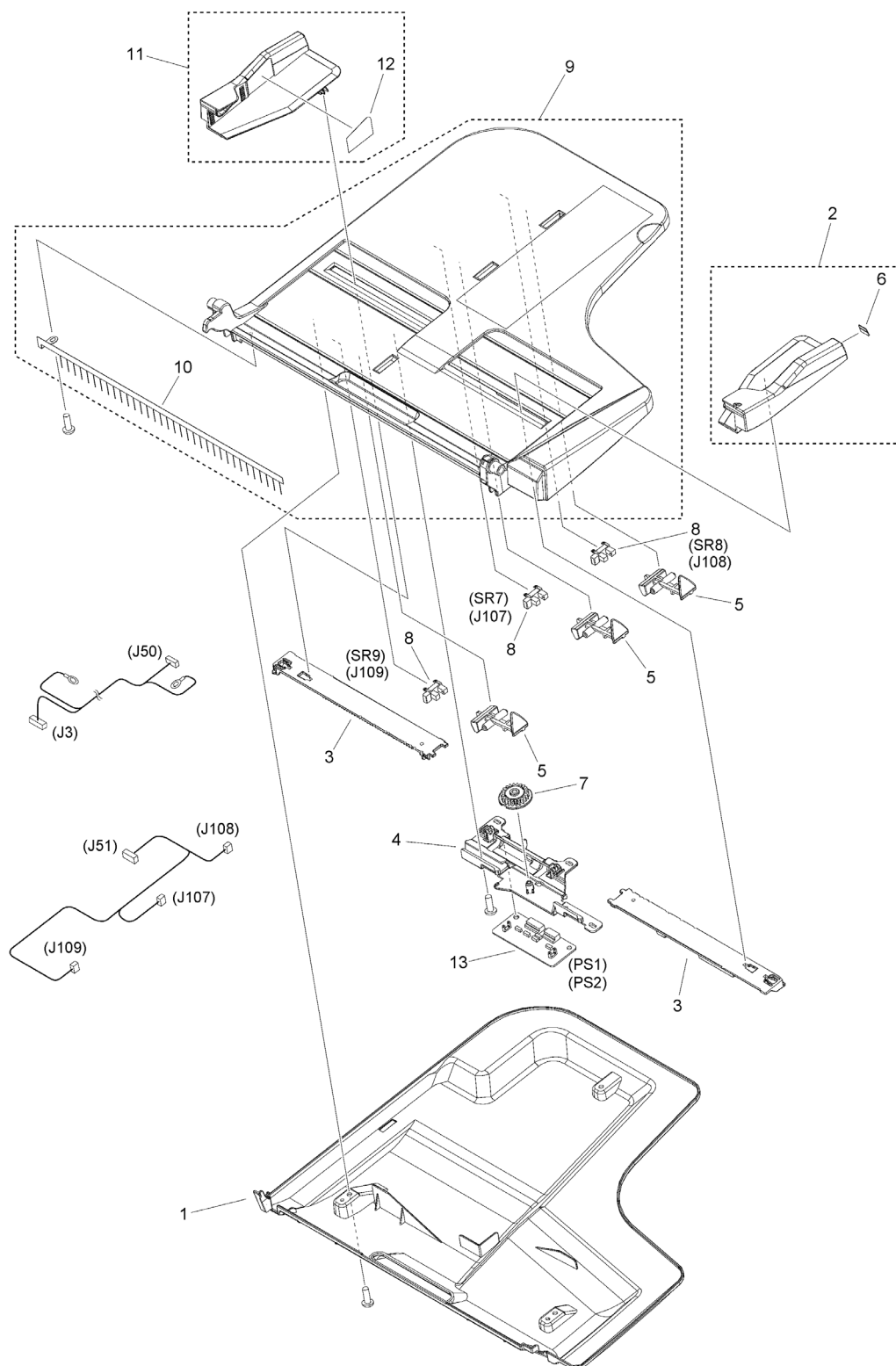
Figure A13 DOCUMENT TRAY ASSEMBLY (ADF model)
