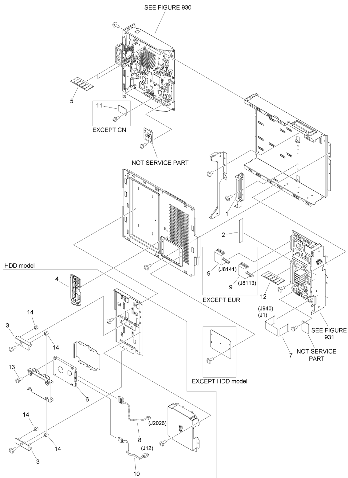
Figure 900 CONTROLLER BOX ASSEMBLY
